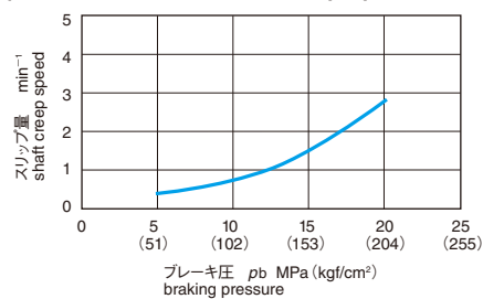
◆保持特性/Shaft creep speed
