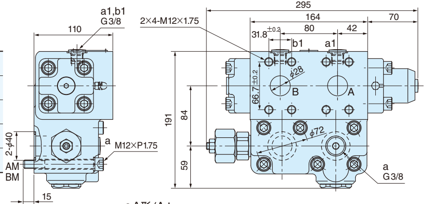
●A形/A type
