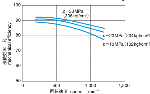
◆起動効率/Starting mechanical efficiency
