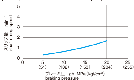
◆保持特性/Shaft creep speed
