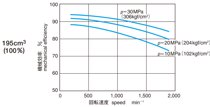
◆機械効率 / Mechanical efficiency (%)
