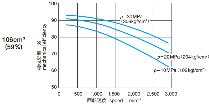
◆起動効率 / Starting mechanical efficiency
